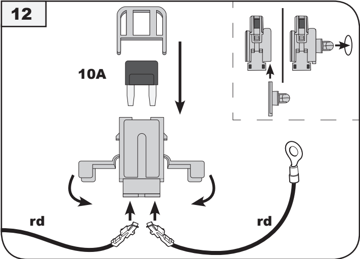
Modul Trail-tec 09-00 LED → Stecker 14 pin E-Satz modul Trail-tec 09-00 LED → socket 14 pin e-kit
