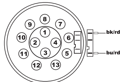
Contact description in 13-pin socket
